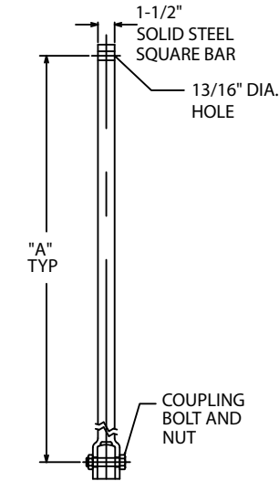
PLAIN EXTENSION
