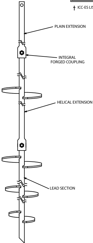
TYPICAL ANCHOR/PIER ASSEMBLY
