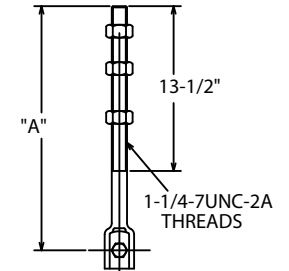
THREADED ADAPTER C150-0032 FOR 1-1/2" SHAFT
