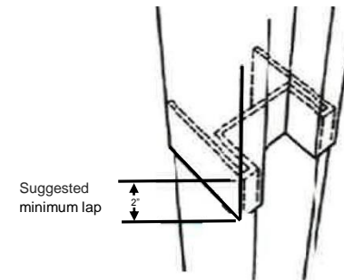
7) As each section is installed, lap as shown in figure 7 until desired length of pile is covered.
